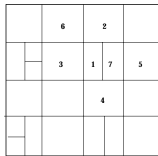
1's coordinate neighbor set = {2,3,4,7} 7's coordinate neighbor set = {1,2,4,5}
