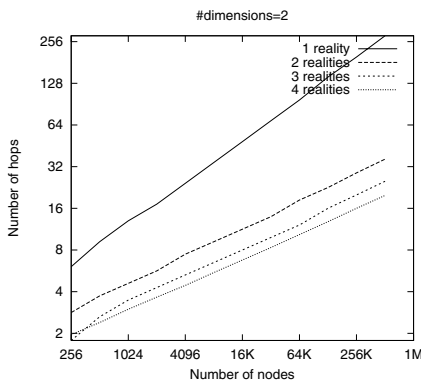
Figure 5: Effect of multiple realities on path length
